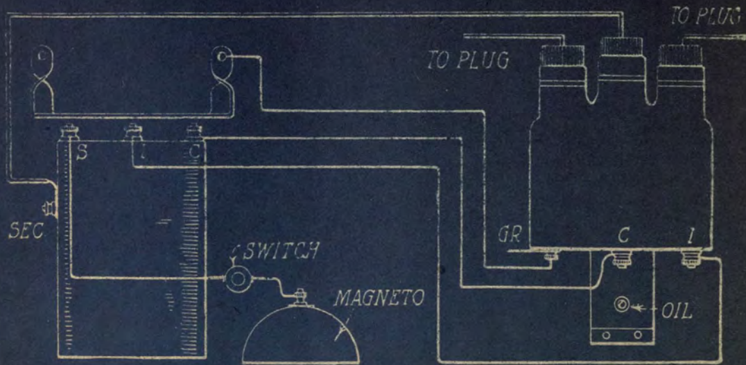
VIBRATOR-LES IGNITION SYSTEM FOR FORD
