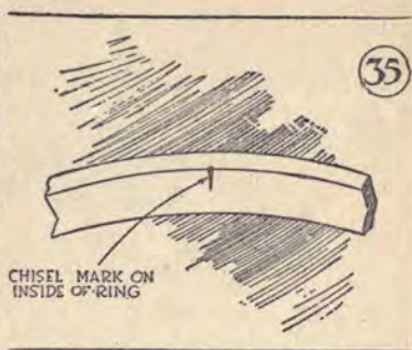
Fig. 35—This chisel mark on the piston ring goes to the top
