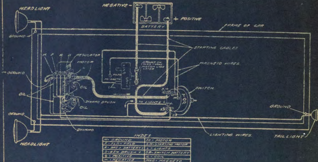
HEINZE-SPRINGFIELD STARTING AND LIGHTING SYSTEM WITH ELECTRO-MAGNETIC REGULATION
