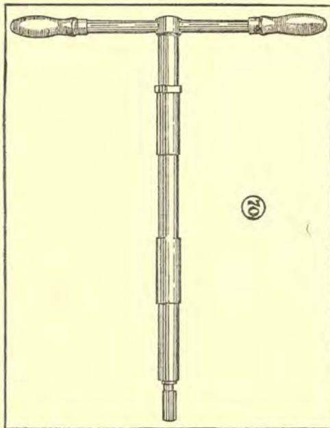
Fig. 70—Line reamer for camshaft bearing
