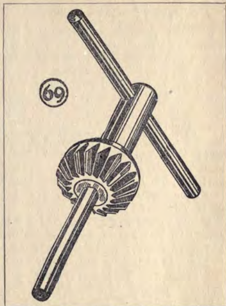
Fig. 69—A plain valve reseater
