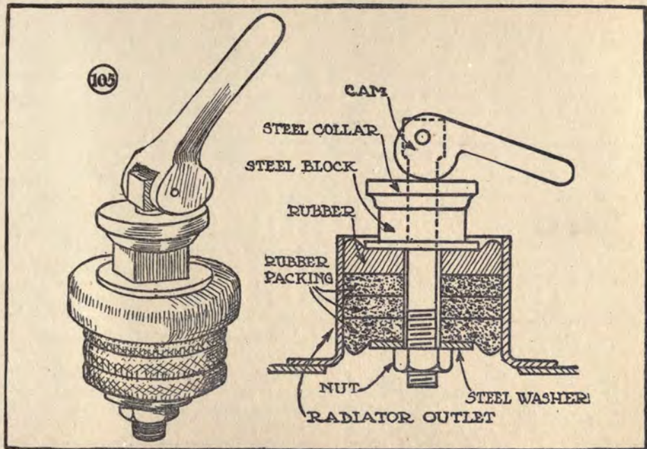
Fig. 105—Rubber compression plug used for making tight joints at inlet
