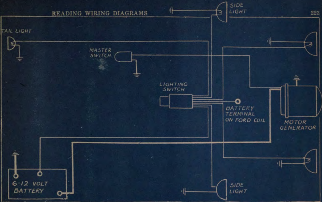
EVEREADY STARTING AND LIGHTING SYSTEM FOR FORD
