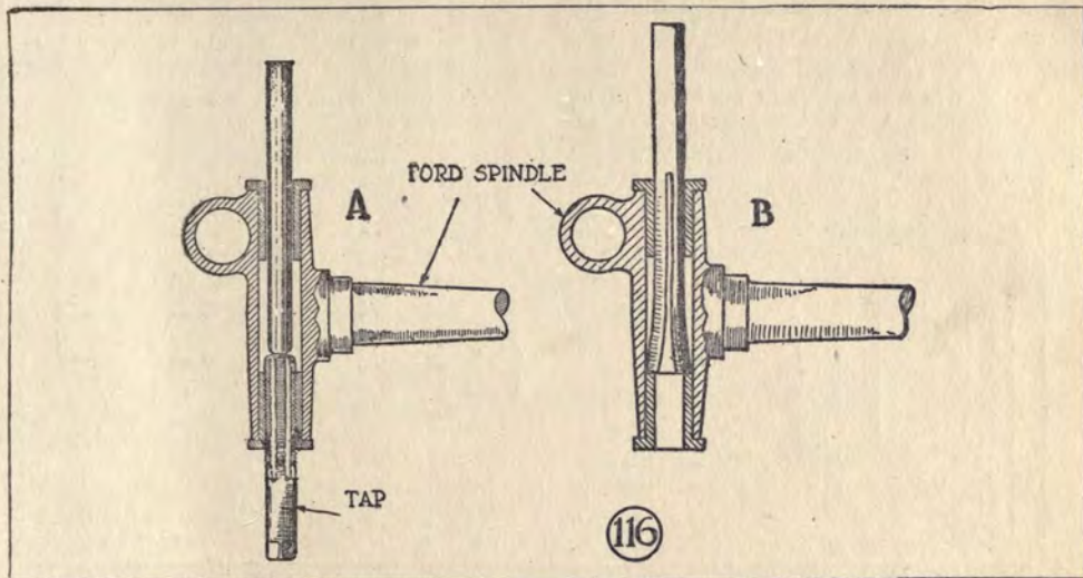
Fig. 116—Two methods of removing spindle body bushings. A shows a tap started in one of the bushings so that an old spindle bolt can be driven against the bottom of the tap, both tap and bushing being driven out. B is a split pin which is compressed to get it in the top bushing, the legs then spreading out so that they will push the other bushing out
