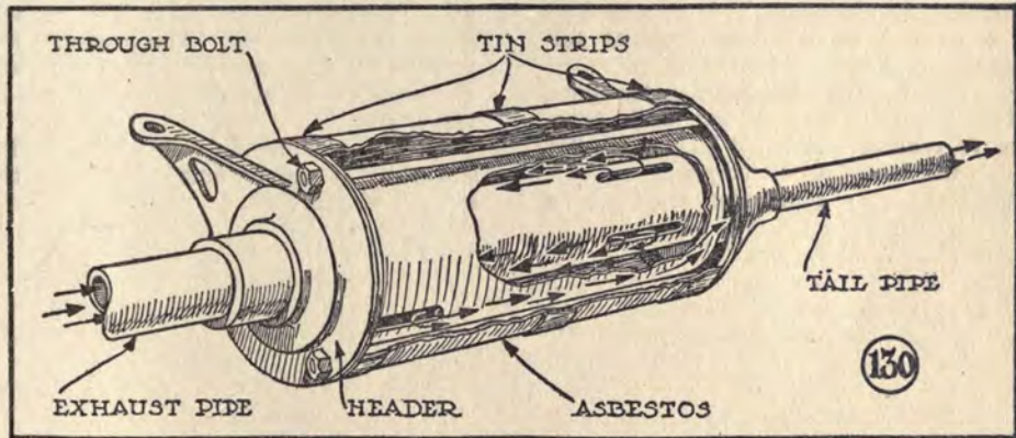
Fig. 130—The muffer is easily disassembled by taking out the three long bolts which will allow all the parts to drop out. The headers have ledges to hold the shells in their proper position, and in re-assembling the slots must be put at the opposite ends of the muffer
