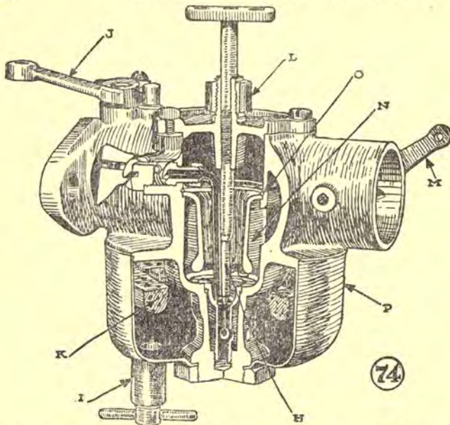
Fig. 74—Section of Holley Model G carbureter. H is needle valve, I drain cock, J throttle lever, K float, L needle valve locknut. M choke throttle lever. N choke tube. O locking ring
