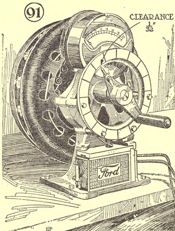
Fig. 91—This coil-unit testing machine is used for testing the units and adjusting the vibrators to the best possible position
