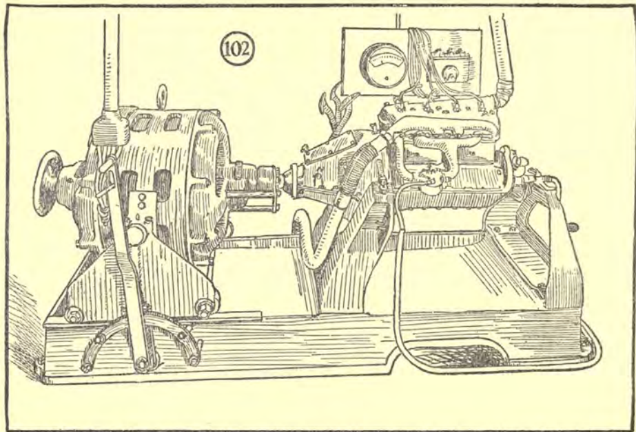
Fig. 102—An electric motor rigged up in connection with an engine testing
