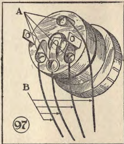
Fig. 97—The switch may cause trouble. A shows possible loose or poorly made connections shorting into switch housing. B shows possible wires grounding at point of entering switch housing or conduit on steering column
