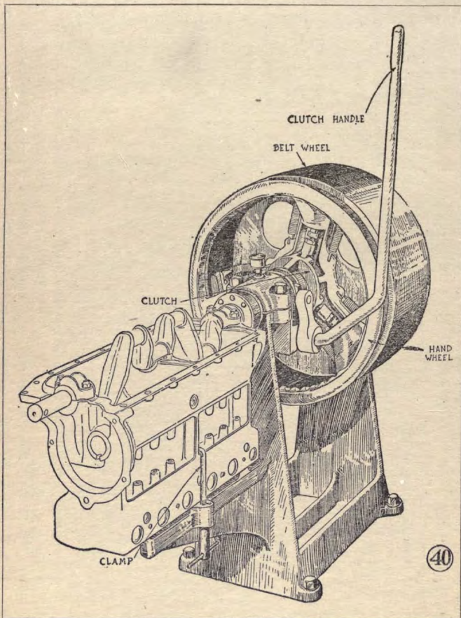
Fig. 40—This is one type of burning-in machine. In this case the block is turned upside down and is clamped in place with two quick-acting clamps
