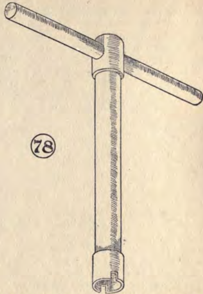
Fig. 78—Slotted tool for removing and replacing the spray nozzle on the Holley carbureter
