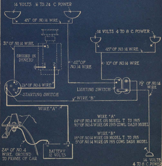
DYNETO STARTING AND LIGHTING SYSTEM FOR FORD 1913-14
