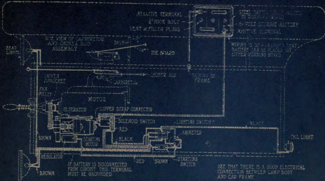
DISCO TWO UNIT STARTING AND LIGHTING SYSTEM FOR FORD
